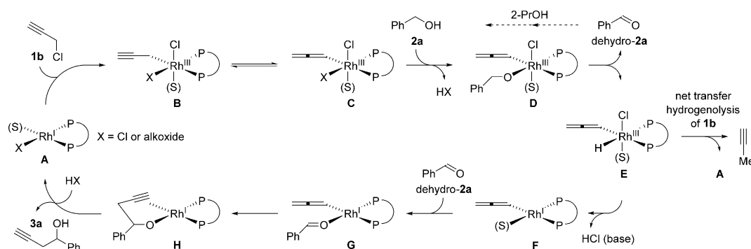
Scheme 1. General catalytic mechanism for rhodium-catalyzed alcohol C-propargylation. [a]
