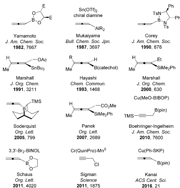
Figure 2. Selected methods for enantioselective carbonyl propargylation. [15–17]
